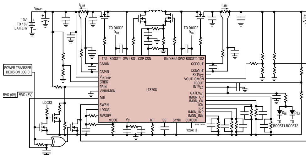
12V Bidirectional Dual Battery System with FHCM and RHCM
