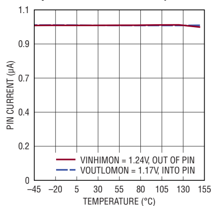
VINHIMON and VOUTLON Pin Hysteresis Current vs Temperature
