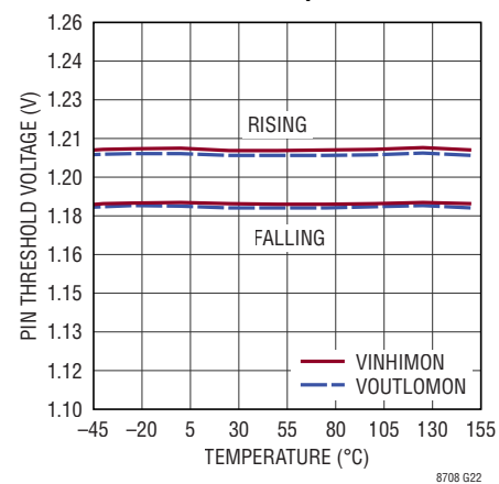
VINHIMON and VOUTLON Pin Thresholds vs Temperature
