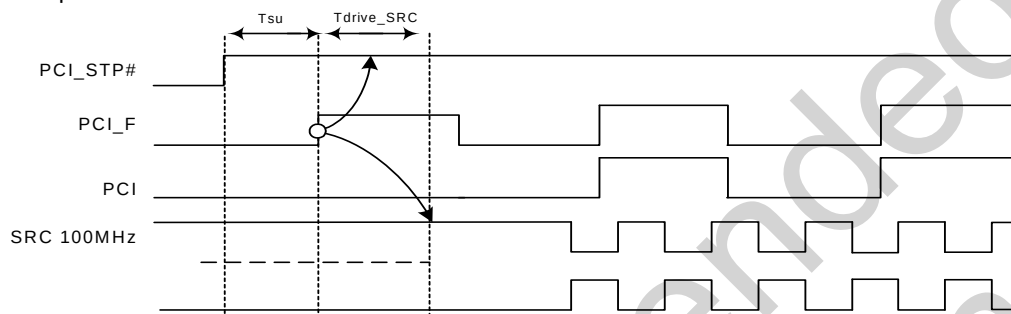
Figure 7. PCI_STP# Deassertion Waveform
