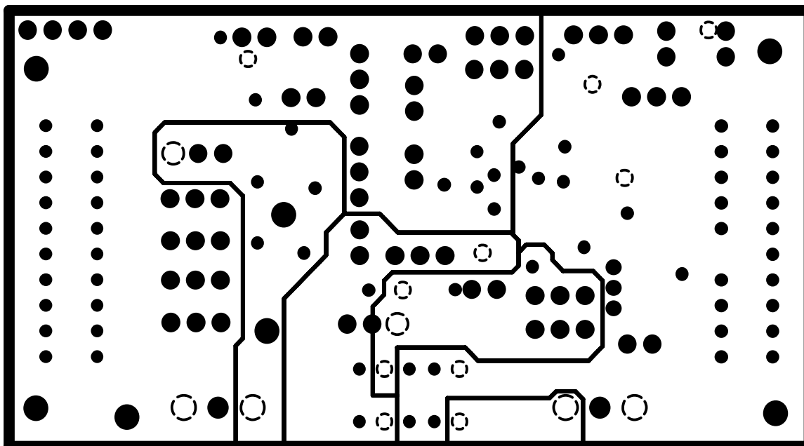
Figure 2–4. Layer 3 (Power Plane)
