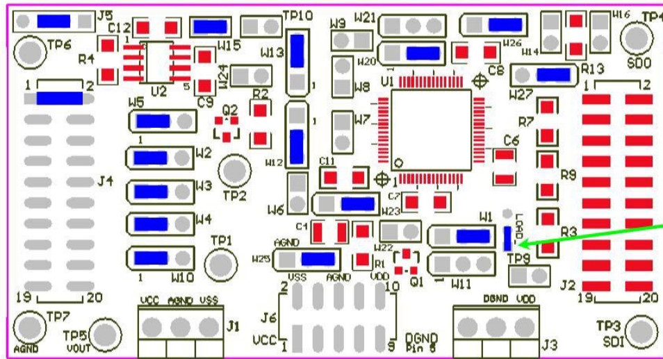
Figure 3–1. DAC7654 EVM Default Jumper Setting
