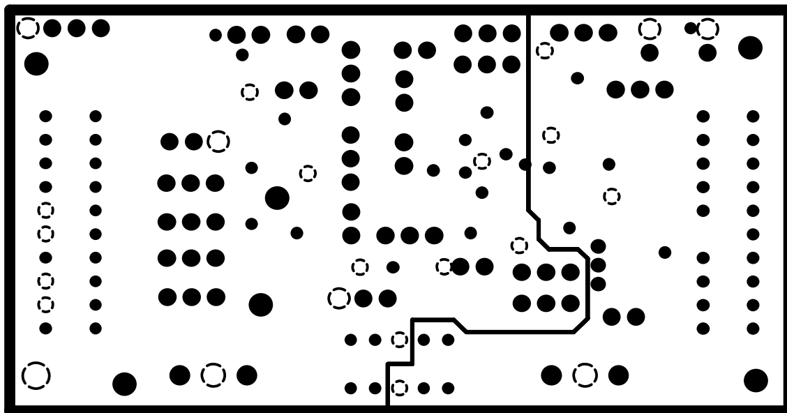
Figure 2–3. Layer 2 (Ground Plane)
