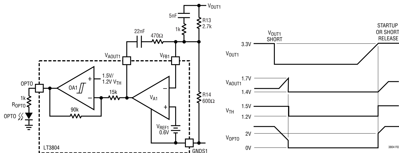
Figure 3. Optocoupler Driver
