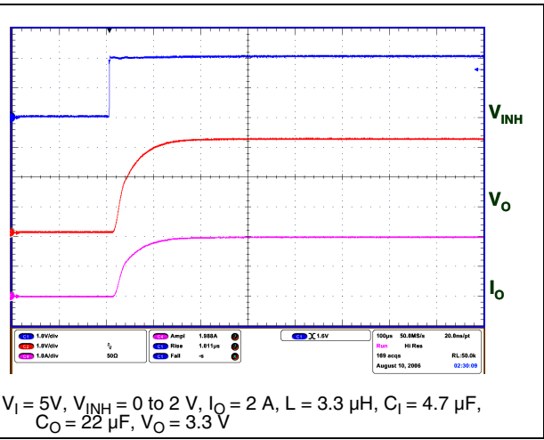
Figure 20. Inhibit transient
