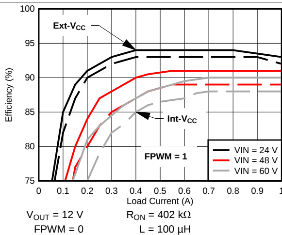
Figure 3. Efficiency at 300 kHz
