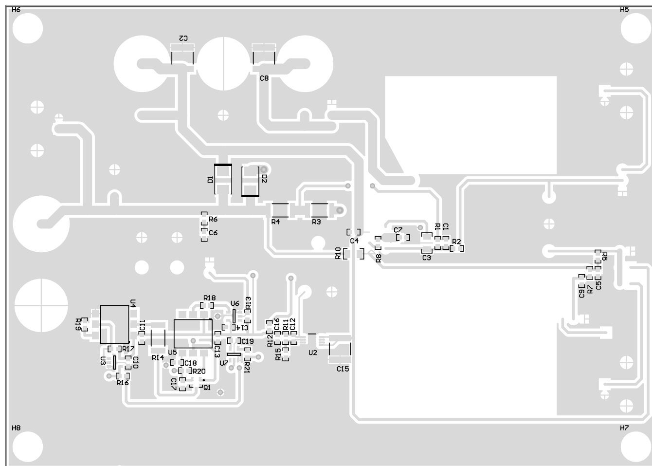
Figure 3. OPA547EVM, OPA548EVM Bottom Layer
