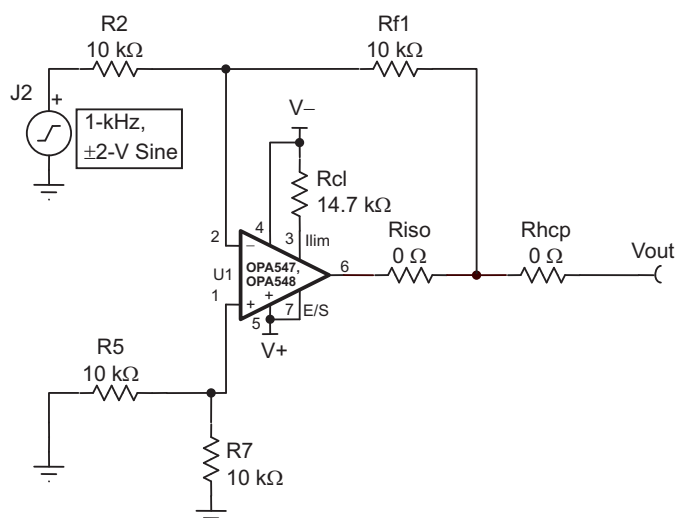
Figure 6. Inverting Amplifier Configuration Schematic
