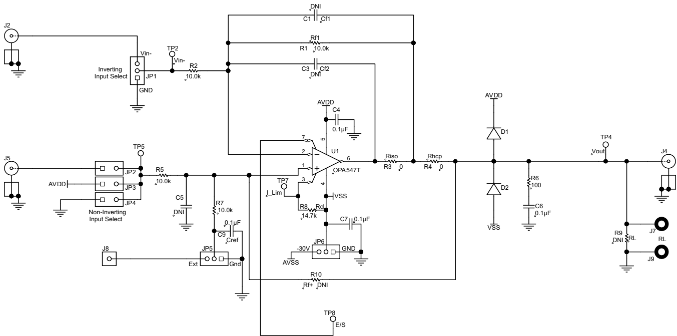
Figure 1. OPA547, OPA548 EVM Schematics
