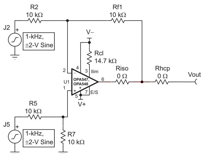
Figure 8. Differential Amplifier Configuration Schematic
