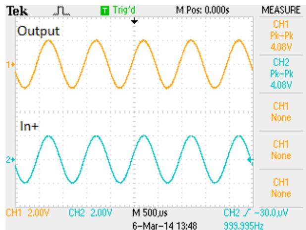
a) Dual-Supply Mode
