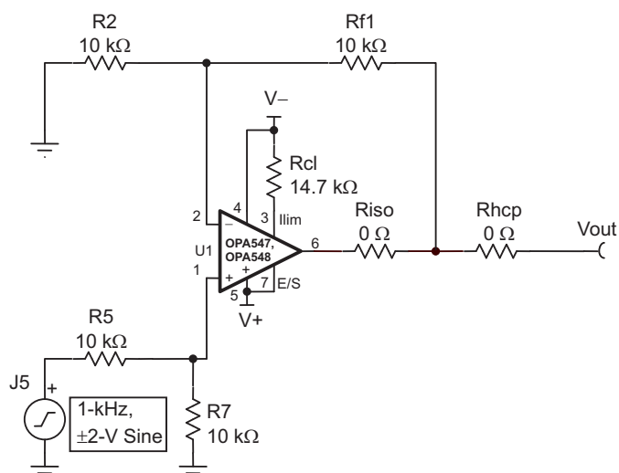
Figure 4. Noninverting Amplifier Configuration Schematic
