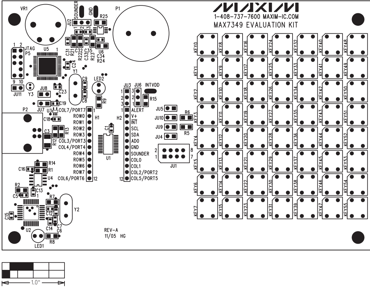
Figure 3. MAX7349 EV Kit Component Placement Guide—Component Side
