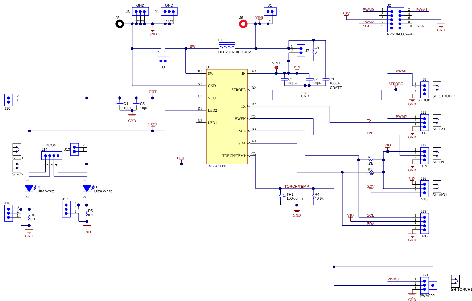
Figure 11. LM3643EVM Schematic
