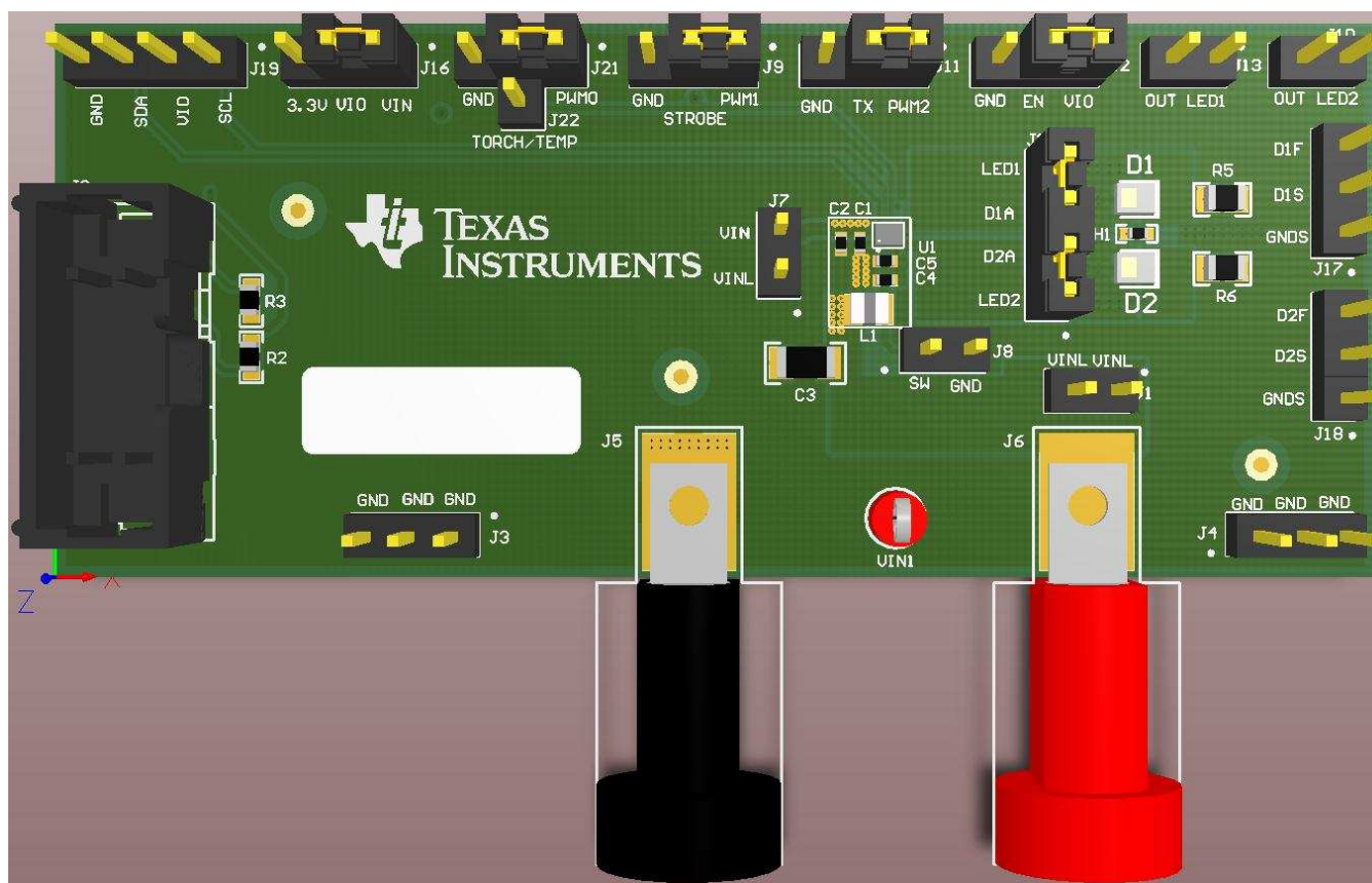
Figure 6. Jumper Configuration
