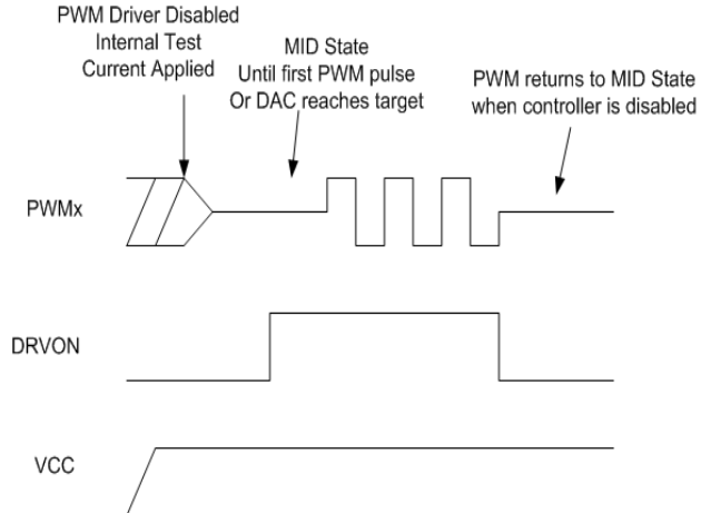
Figure 15. Soft-Start Sequence
