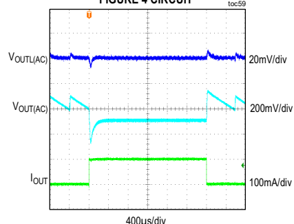
MAX17671F, STEP-DOWN CONVERTER LOAD TRANSIENT ON 3.3V LINEAR REGULATOR OUTPUT, FIGURE 4 CIRCUIT
