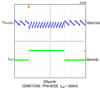
MAX17670E, 3.3V OUTPUT LOAD TRANSIENT BETWEEN 1mA AND 50mA FIGURE 5 CIRCUIT
