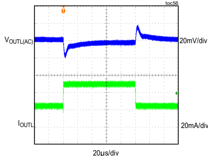
MAX17671F, 3.3V LINEAR REGULATOR LOAD TRANSIENT BETWEEN 25mA AND 50mA FIGURE 6 CIRCUIT
