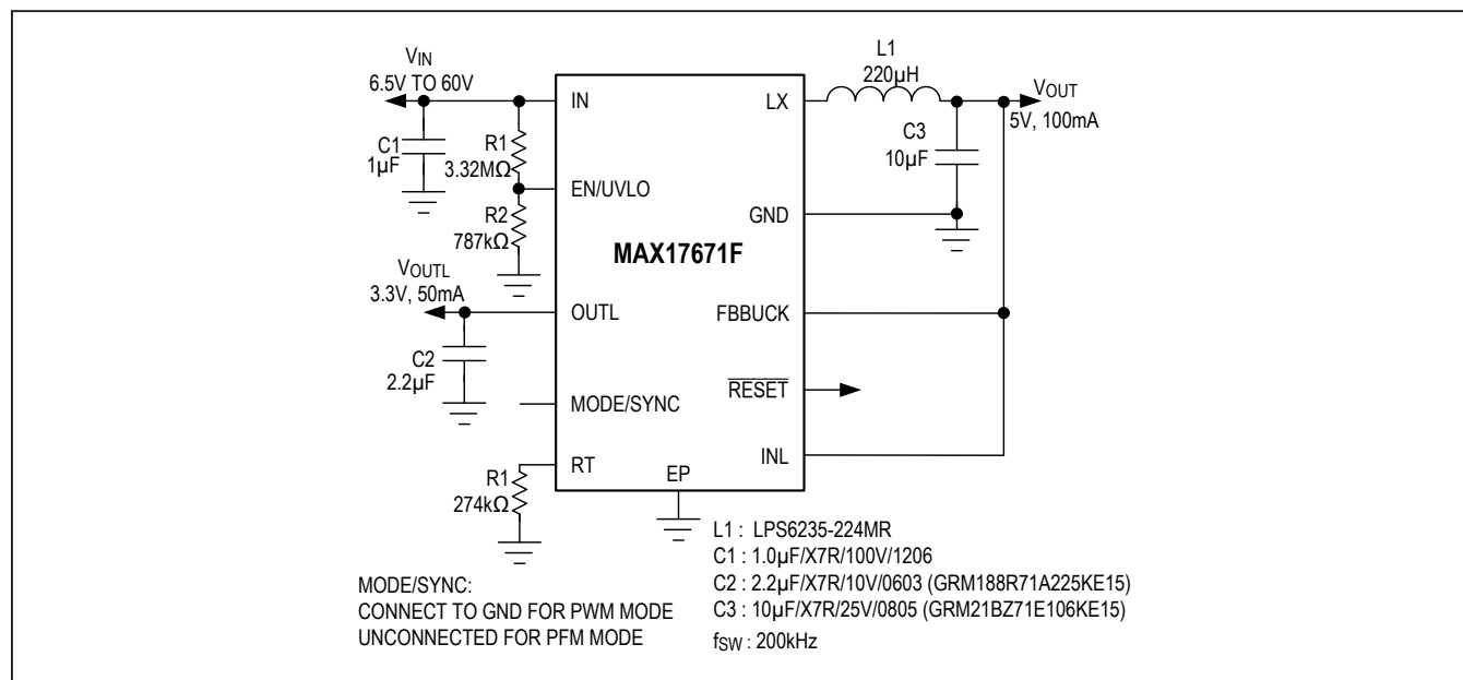
Figure 4. Fixed 5V Step-Down Converter Output at 200kHz Switching Frequency and 3.3V Linear Regulator Output
