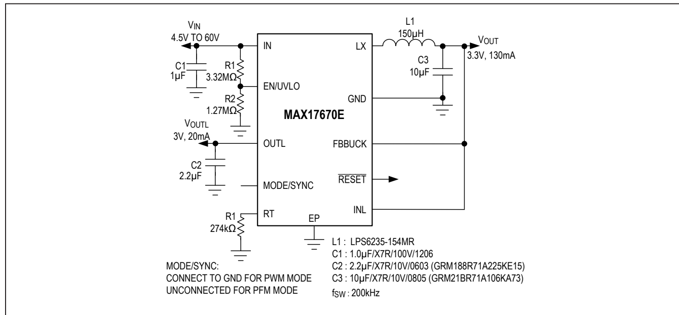
Figure 5. Fixed 3.3V Step-Down Converter Output at 200kHz Switching Frequency and 3.0V Linear Regulator Output
