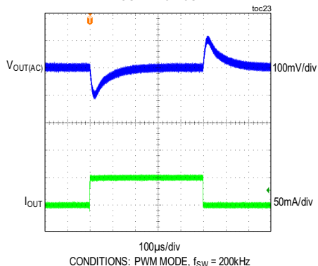
MAX17671F, 5V OUTPUT LOAD TRANSIENT BETWEEN 0mA AND 50mA FIGURE 4 CIRCUIT
