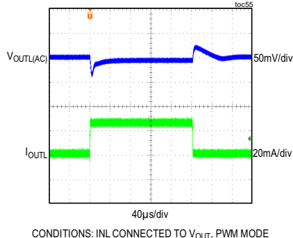
MAX17671F, 3.3V LINEAR REGULATOR LOAD TRANSIENT BETWEEN 1mA AND 25mA FIGURE 6 CIRCUIT
