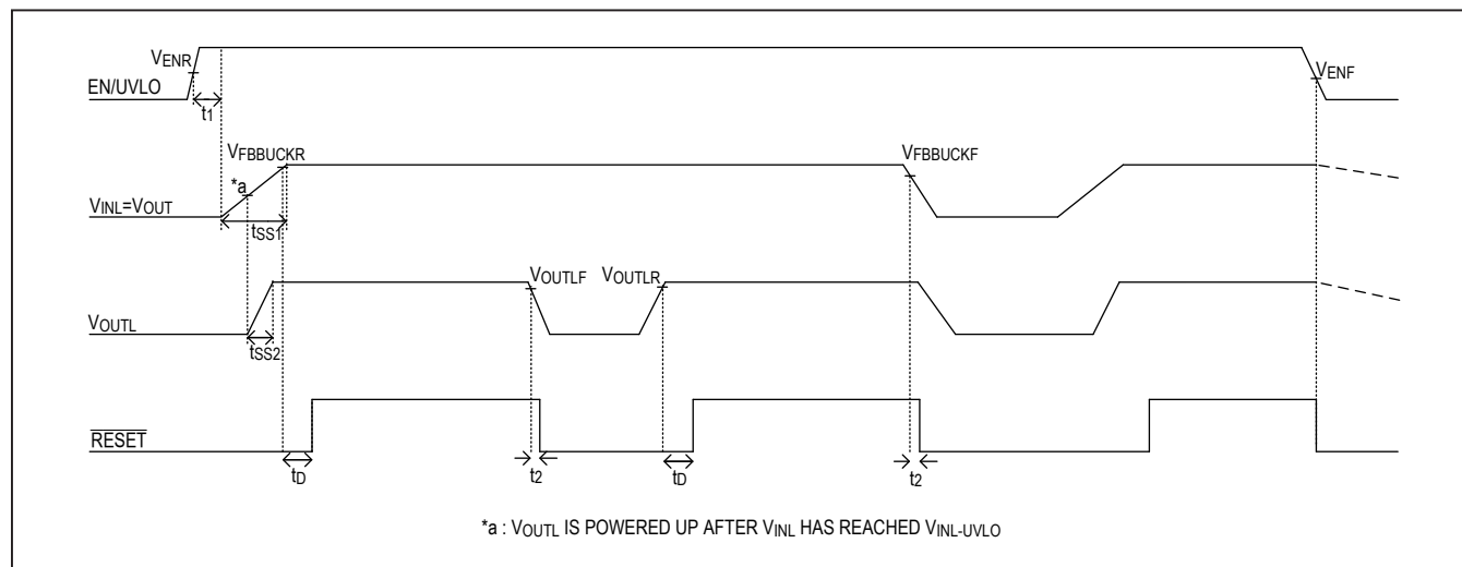
Figure 1. \overline{\text{RESET}} Output Logic Diagram
