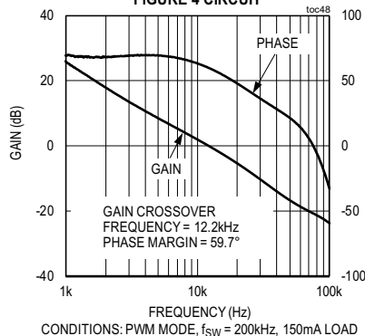
MAX17671F, 5V OUTPUT CLOSED LOOP BODE PLOT FIGURE 4 CIRCUIT
