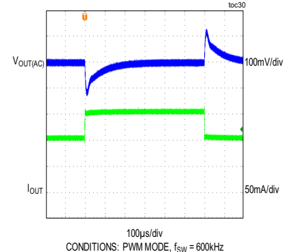
MAX17670E, 3.3V OUTPUT LOAD TRANSIENT BETWEEN 0mA AND 50mA FIGURE 7 CIRCUIT
