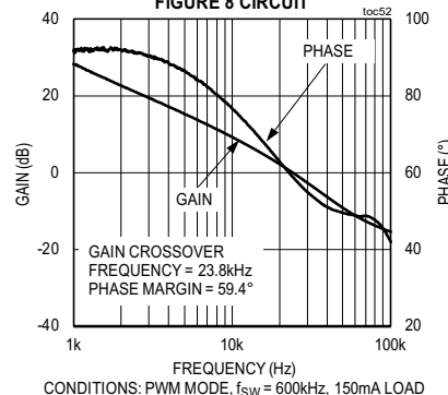
MAX17672C, 5V OUTPUT CLOSED LOOP BODE PLOT FIGURE 8 CIRCUIT
