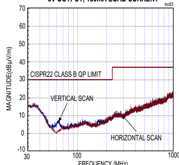
RADIATED EMISSIONS PLOT 5V OUTPUT, 150mA LOAD CURRENT
