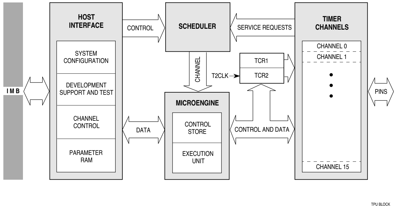
Figure 7-1 TPU Block Diagram
