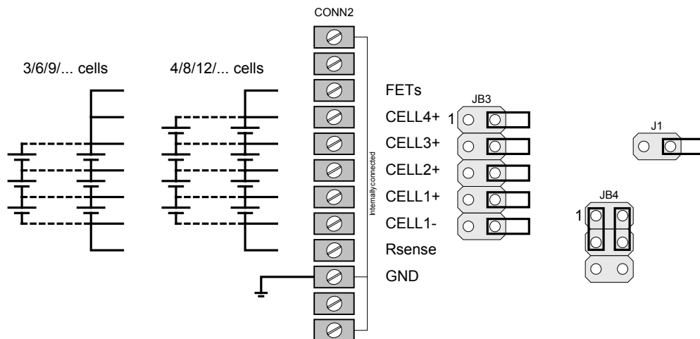
Figure 2-4. Connecting battery cells to CONN2.
