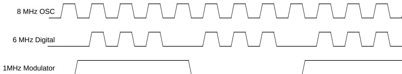
Figure 13. Clock Generation
