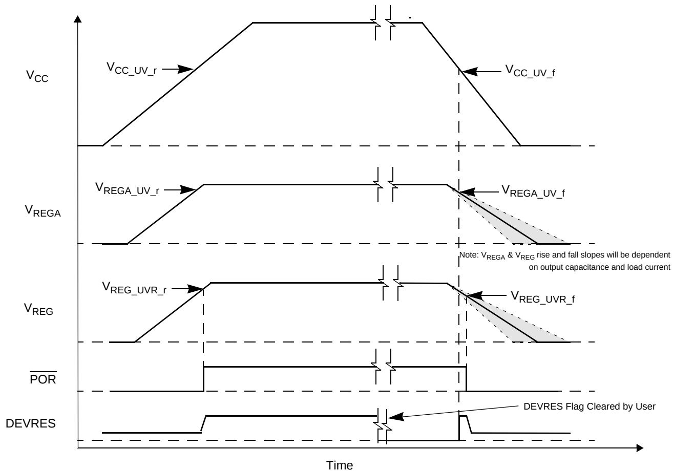
Figure 6. Power-Up Timing
