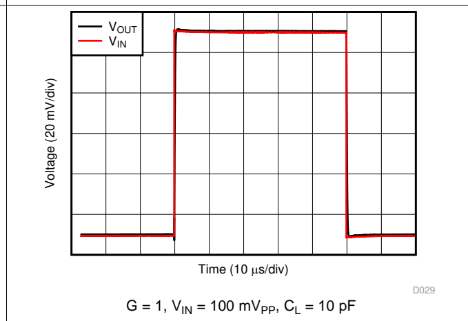
Figure 22. No Phase Reversal
