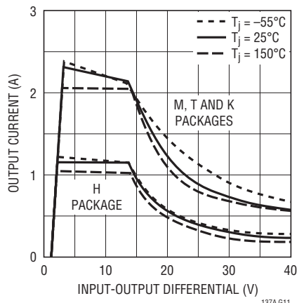
Current Limit
