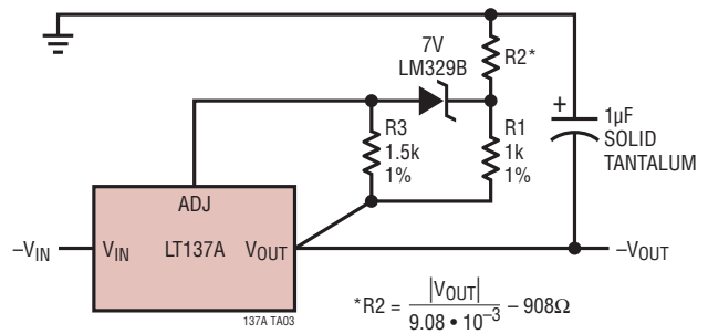
High Stability Regulator
