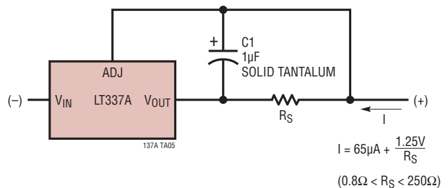
Current Regulator
