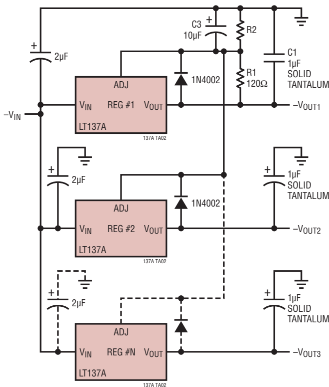
Multiple Tracking Regulators
