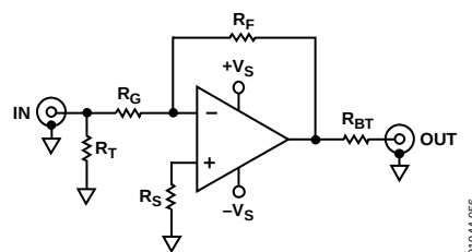
Figure 57. Inverting Configuration
