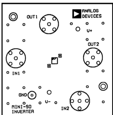
Figure 62. Inverter MSOP Board Layout (Silkscreen)
