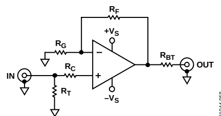
Figure 59. Noninverting Configuration
