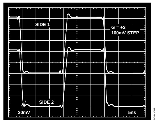
Figure 9. 1 V Step Response, G = +2
