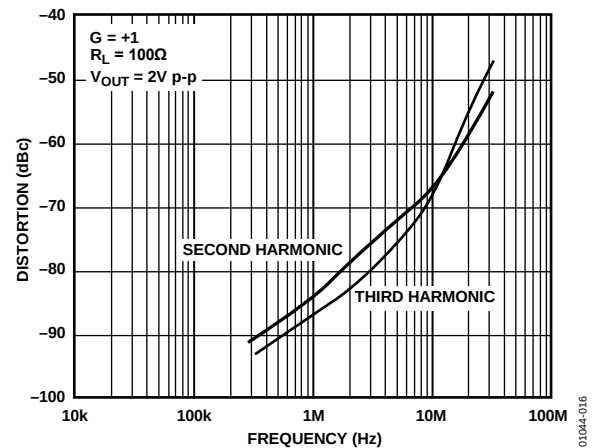
Figure 17. Distortion vs. Frequency, G = +1 , R_L = 100\text{ }\Omega
