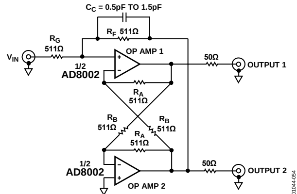
Figure 54. Differential Line Driver
