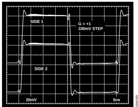
Figure 6. 100 mV Step Response, G = +1
