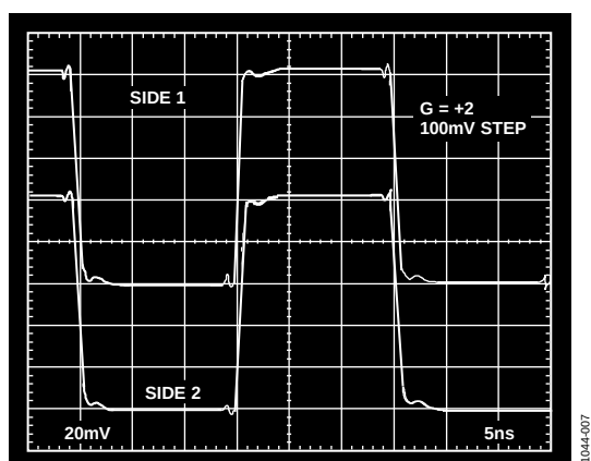
Figure 8. 100 mV Step Response, G = +2
