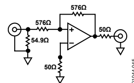
Figure 46. 100 mV Step Response, G = -1
