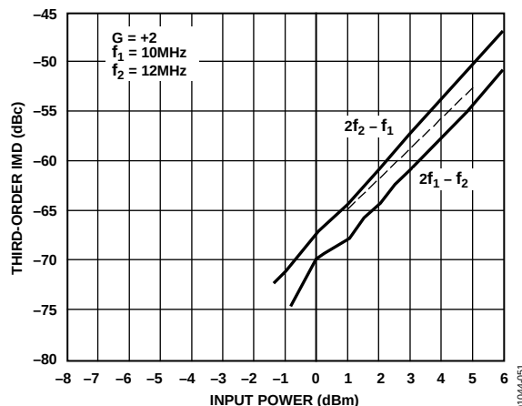
Figure 52. Third-Order IMD vs. Input Power; f_1 = 10 \text{ MHz} , f_2 = 12 \text{ MHz}
