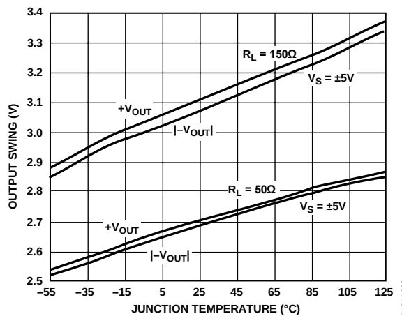
Figure 23. Output Swing vs. Junction Temperature
