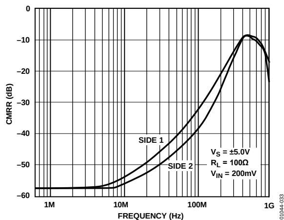
Figure 34. CMRR vs. Frequency (See Figure 45)
