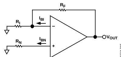
Figure 49. Output Offset Voltage
