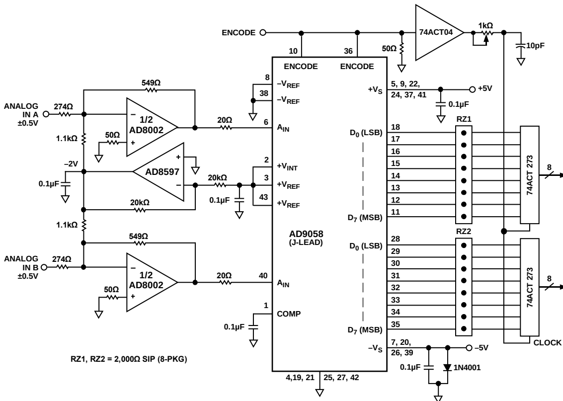
Figure 55. AD8002 Driving a Dual ADC
