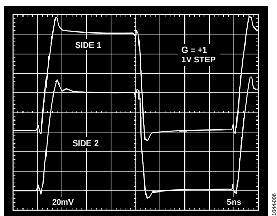
Figure 7. 1 V Step Response, G = +1
