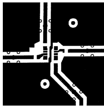
Figure 65. Noninverter SOIC Board Layout (Component Layer)
