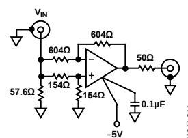
Figure 45. CMRR Test Circuit (See Figure 34)
