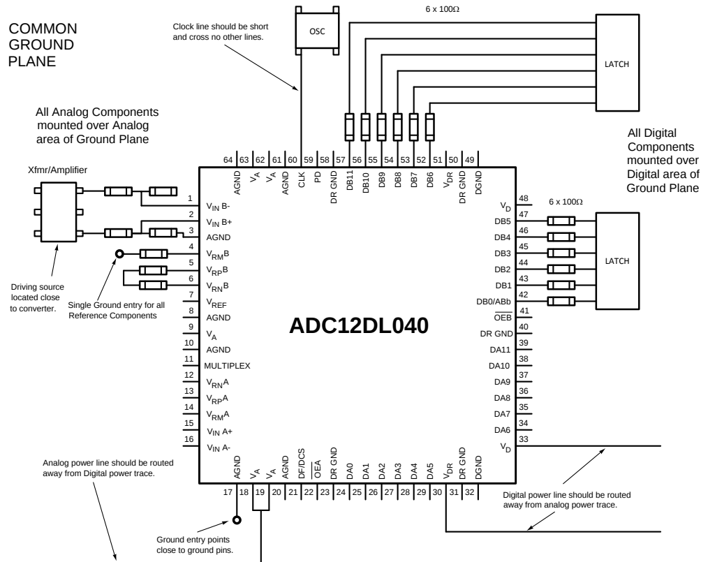
Figure 40. Example of a Suitable Layout
