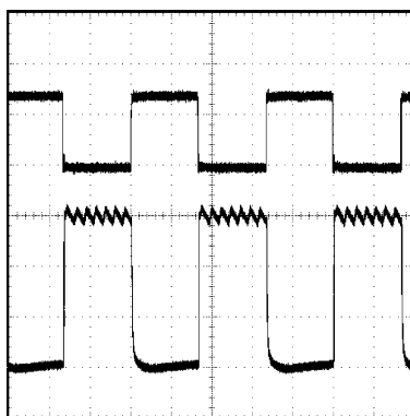
Figure 5. 30kHz PWM Dimming Waveform Showing Inductor Ripple Current I_LED = 6A nominal, V_IN = 3.3V, V_EE = -12V Top trace: DIM input, 2V/div, DC Bottom trace: I_LED, 2A/div, DC T = 10μs/div
