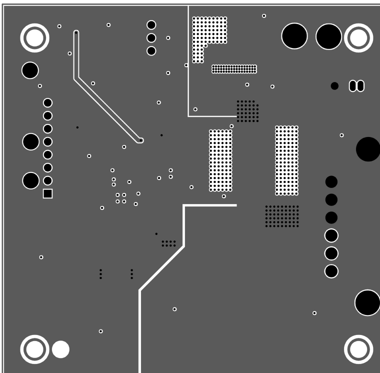
Figure 8. Lower Middle Layer
