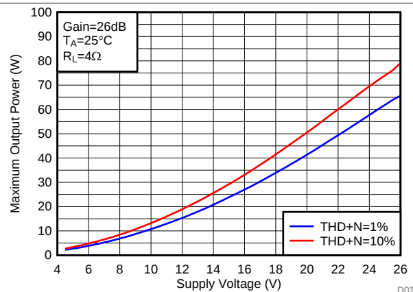
Figure 12. Maximum Output Power (BTL) vs Supply Voltage
