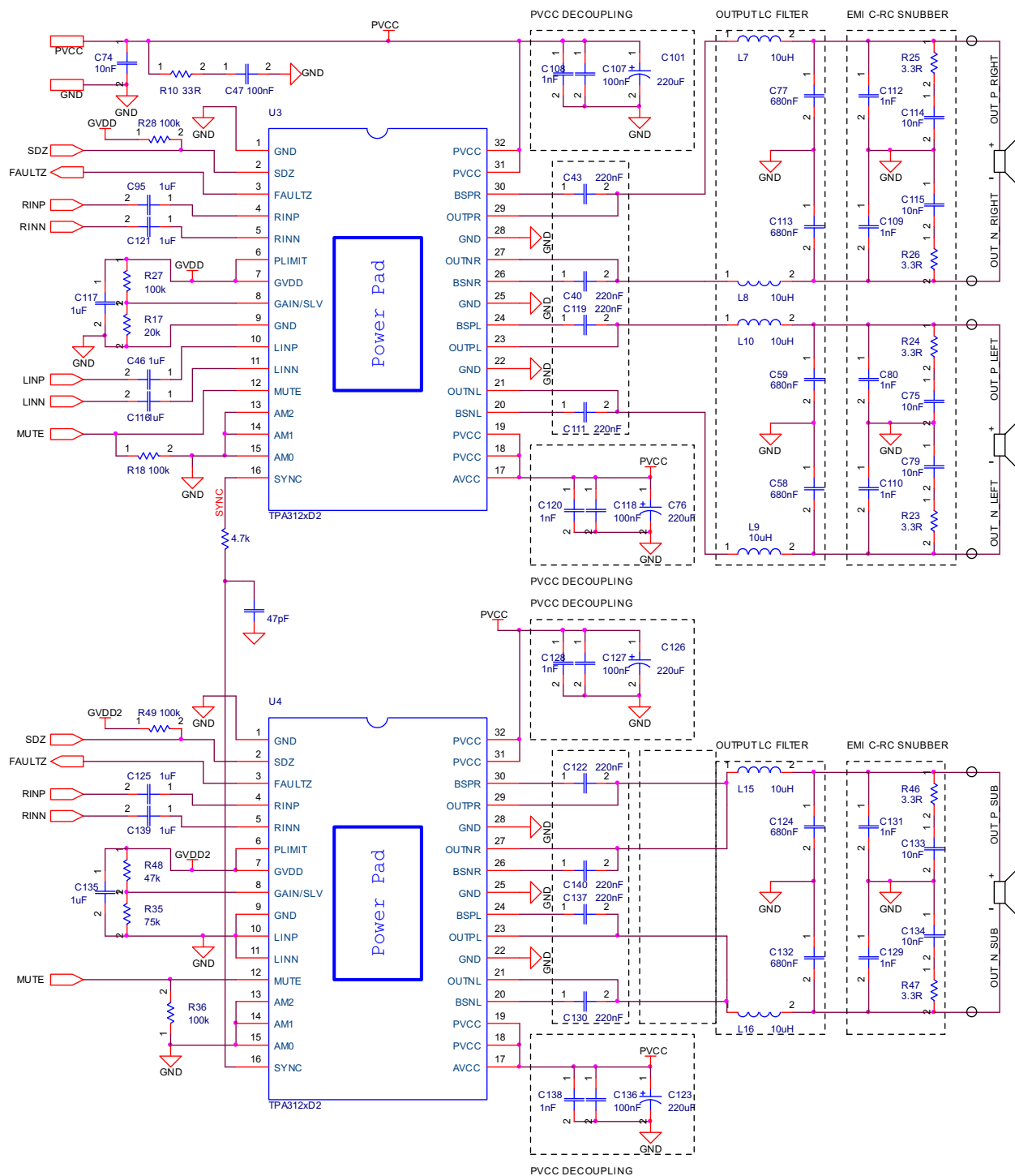
Figure 36. TPA312xD2 Schematic
