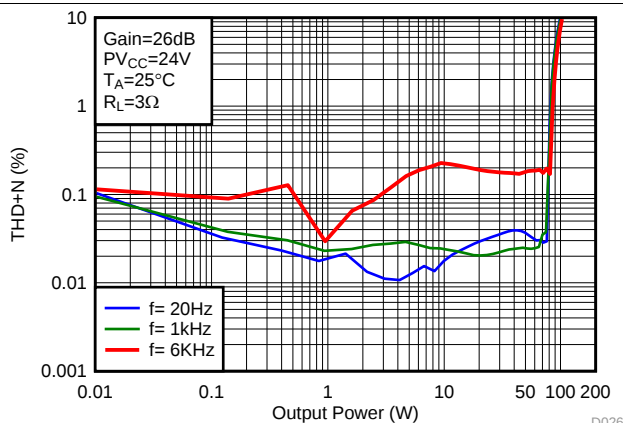
Figure 23. Total Harmonic Distortion + Noise (PBTL) vs Output Power
