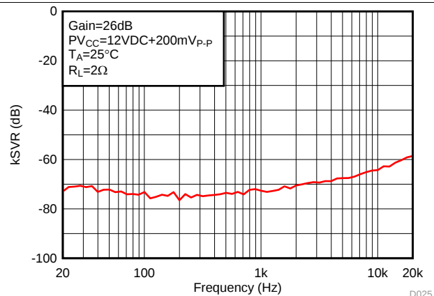
Figure 22. Supply Ripple Rejection Ratio (PBTL) vs Frequency
