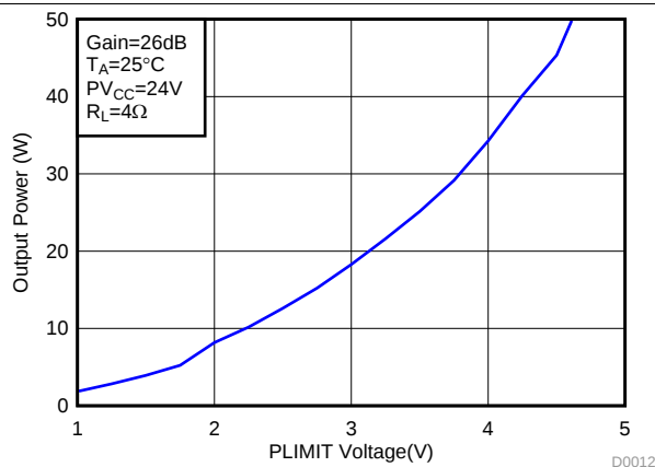
Figure 9. Output Power (BTL) vs Plimit Voltage
