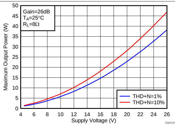
Figure 11. Maximum Output Power (BTL) vs Supply Voltage
