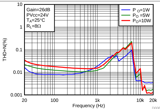
Figure 3. Total Harmonic Distortion + Noise (BTL) vs Frequency
