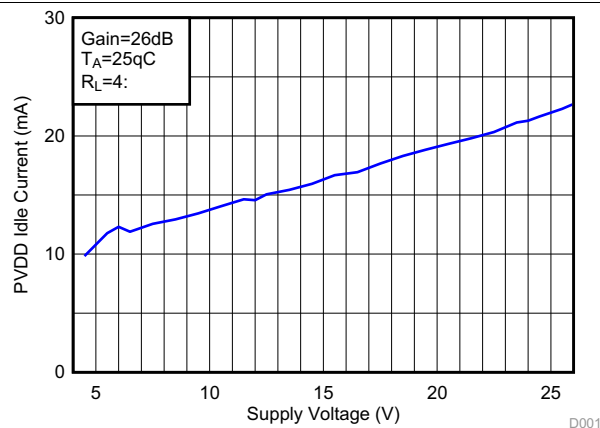
Figure 1. Idle Current vs PVCC
