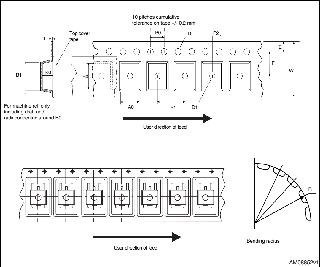
Figure 27. PPAK tape
