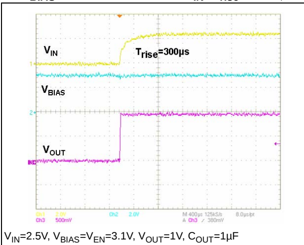
Figure 21. V_{IN} start-up transient response ( V_{BIAS} startup before than V_{IN} ) T_{rise} = 300 \mu s
