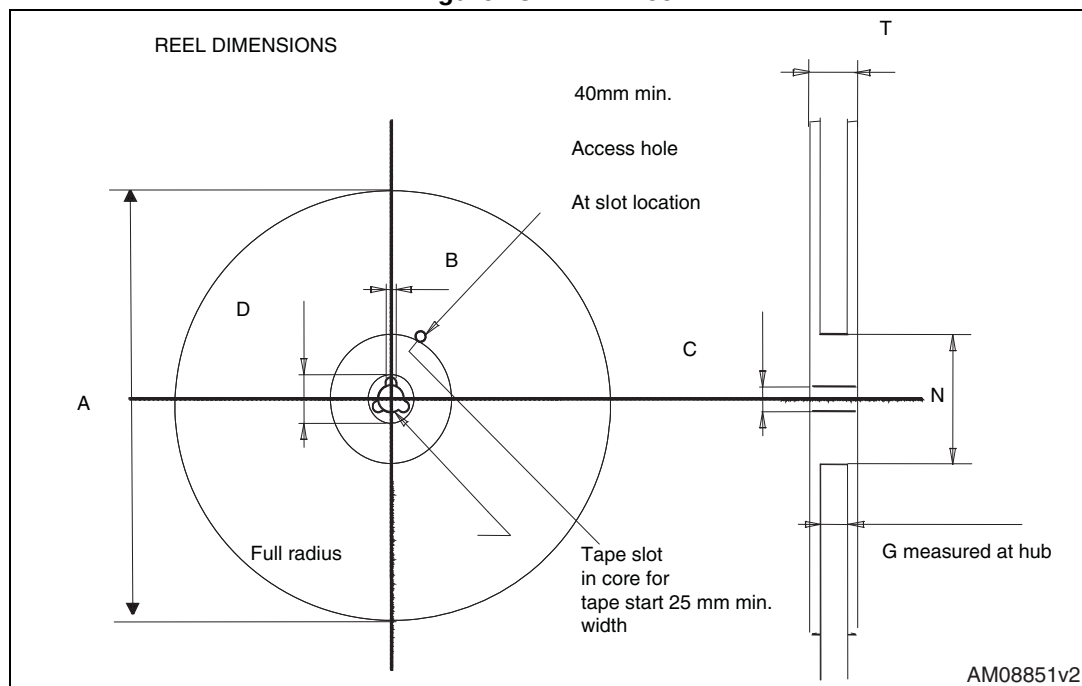
Figure 28. PPAK reel
