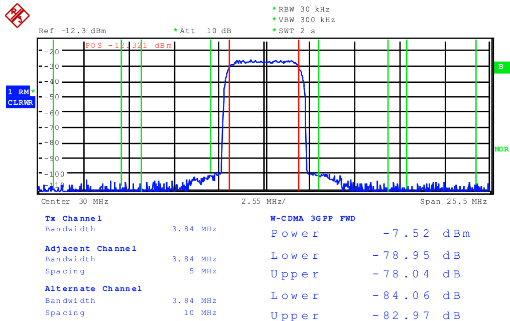
Figure 14. DAC348x Transformer Coupled Output at 30MHz IF
