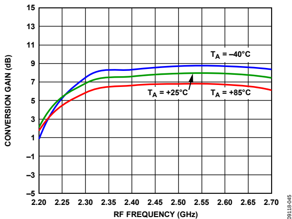
Figure 46. Power Conversion Gain vs. RF Frequency at 3.3 V
