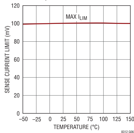
SENSE Pin Threshold Current vs Temperature
