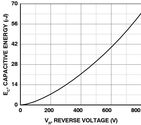
Figure 7. Capacitive Stored Energy
