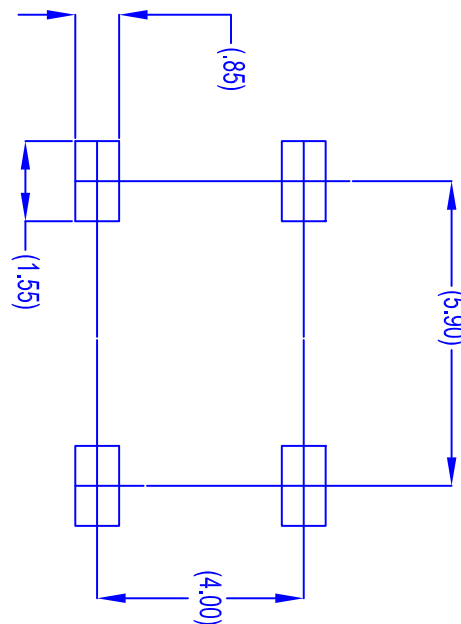
LAND PATTERN RECOMMENDATION
