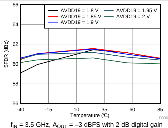
Figure 34. Spurious-Free Dynamic Range vs AVDD19 Supply and Temperature
