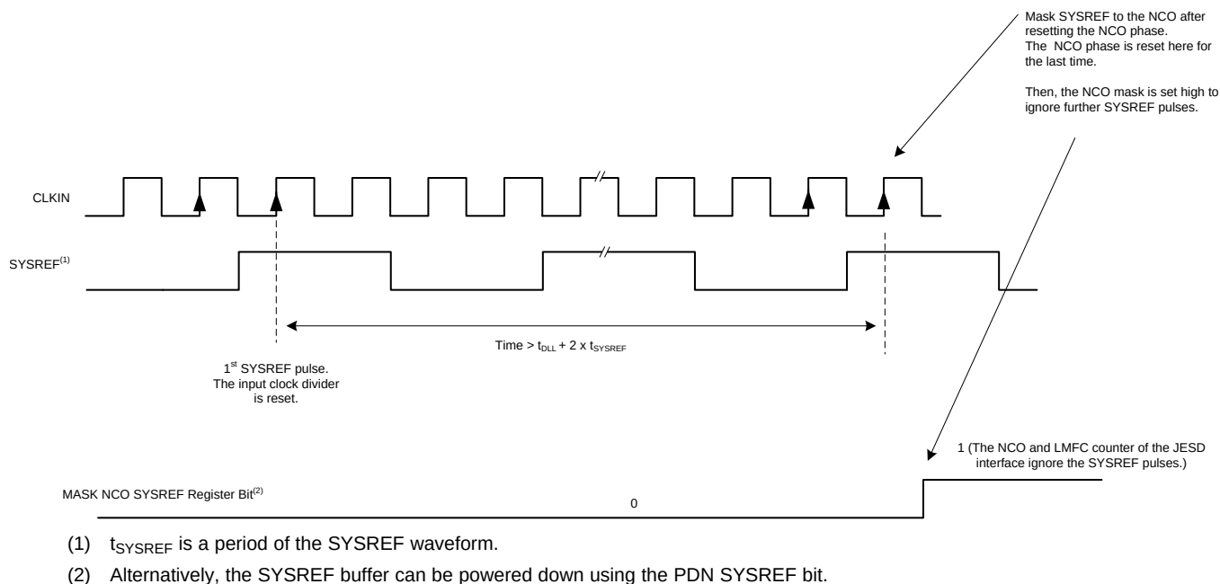
Figure 72. SYSREF Used as a Periodic Waveform
