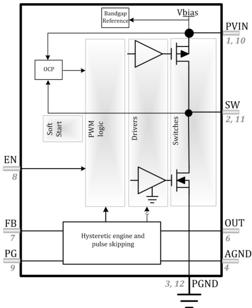
Figure 3: Block Diagram
