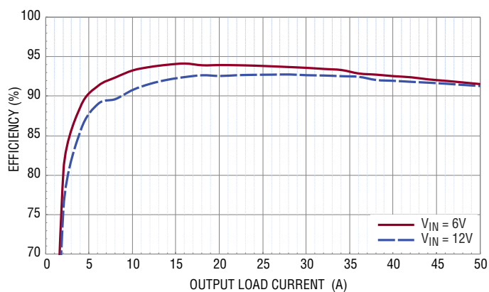
Figure 6. Efficiency vs Load Current on CH1 (CH0 is Disabled, RUNP is ON)
