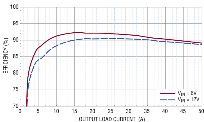
Figure 5. Efficiency vs Load Current on CH0 (CH1 is Disabled, RUNP is ON)
