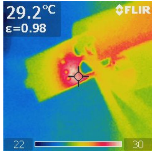
Figure 9. Case Temperature of NSR05F40NX5G in Operation at 25°C, 150 mA 34 V Output
