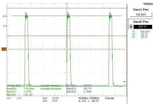
Figure 8. NSR05F30QNX5G on Day 5 at 25°C
