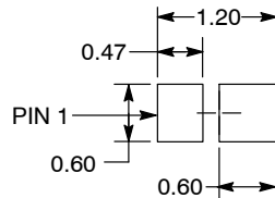
RECOMMENDED SOLDER FOOTPRINT*
