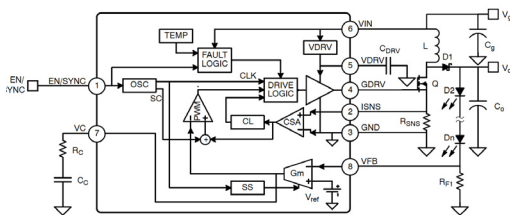
Figure 4. Simplified Typical Single Channel Converter
