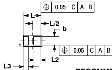
RECOMMENDED SOLDER FOOTPRINT*
