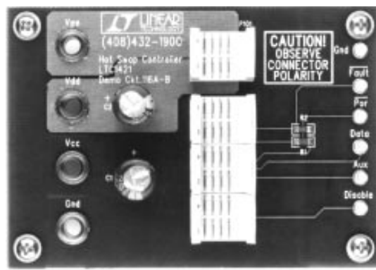
DC116B PHOTO
