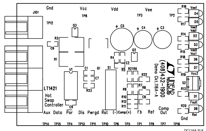
Silkscreen Top
