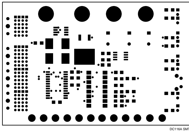
Solder Mask Top
