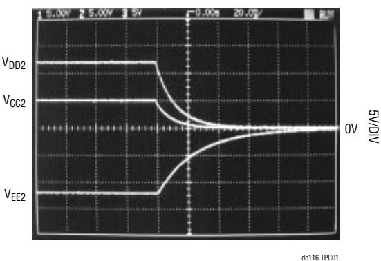
Figure 2. Live Removal from the System Backplane
