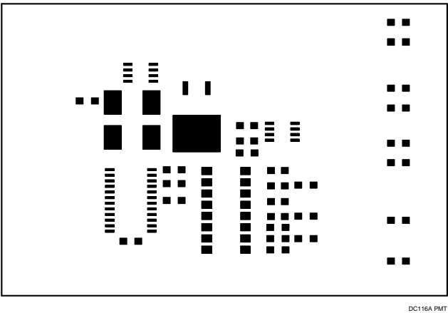
Paste Mask Top
