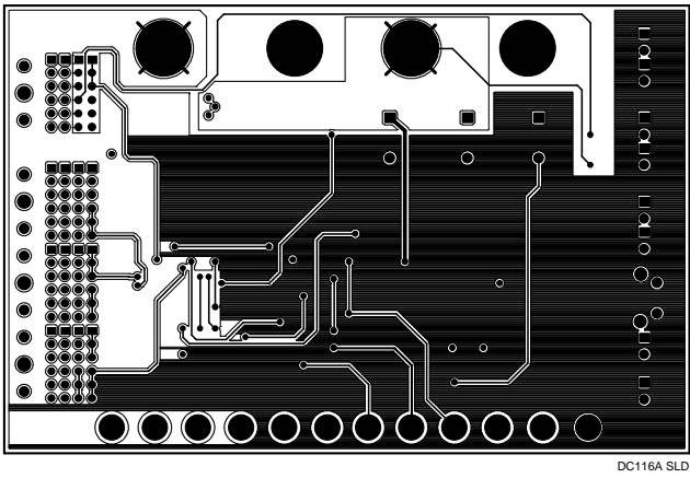
Solder Side
