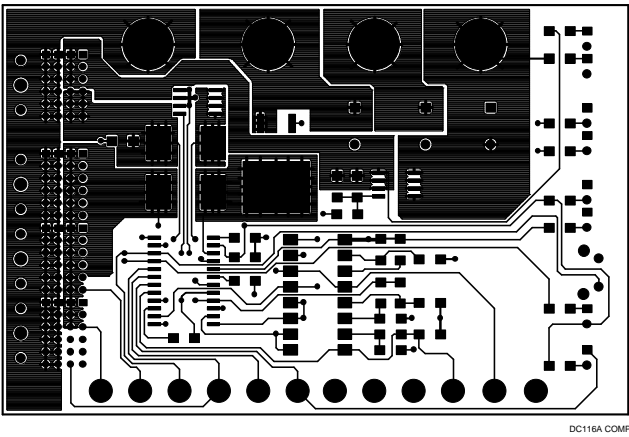
Component Side
