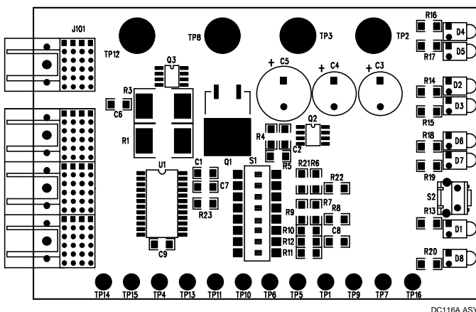
Assembly Top
