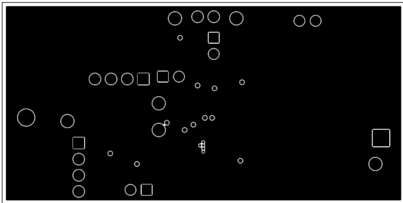
Figure 4. Layer 2
