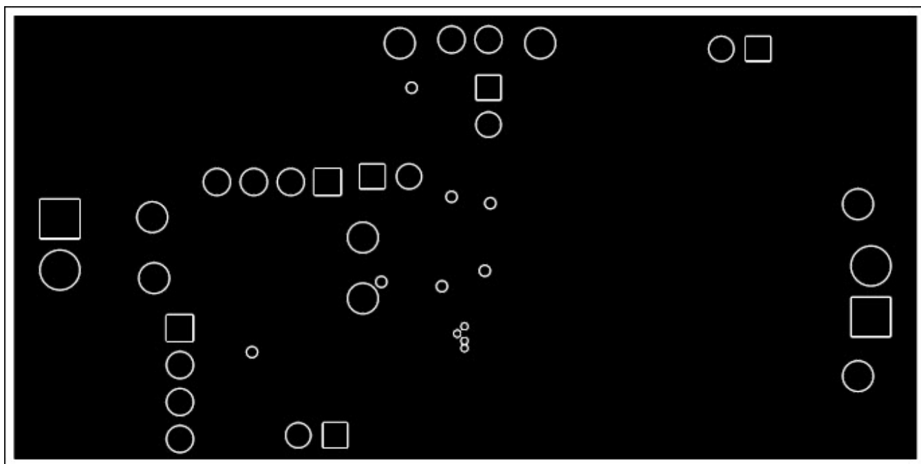
Figure 5. Layer 3
