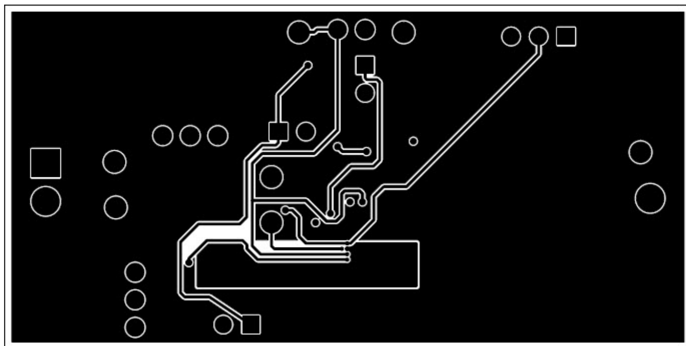
Figure 6. Bottom Layer
