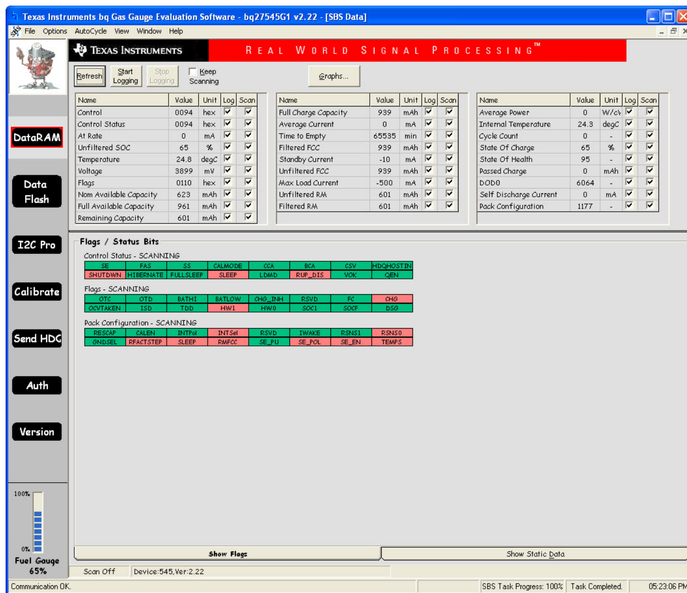
Figure 9. DataRAM Screen
