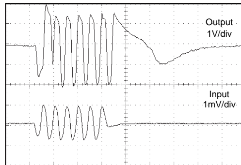
OVERLOAD RECOVERY (Differential, V_{\text{CA\_CTRL}} = 3.0\text{V} , \text{MGS} = 111 )
