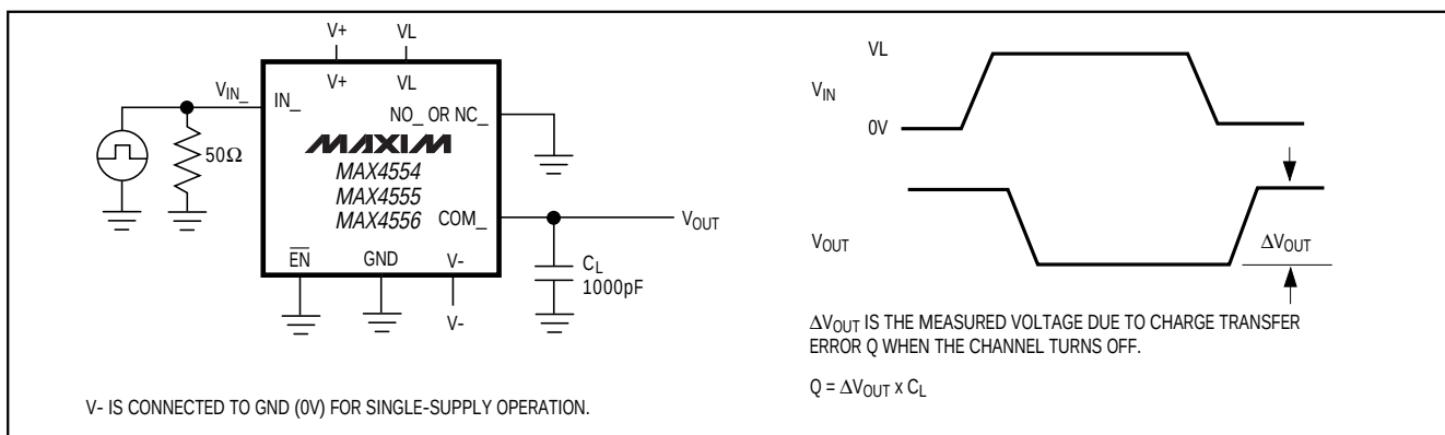
Figure 13. Charge Injection
