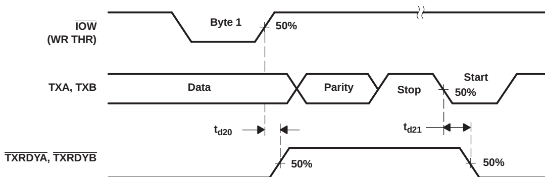
Figure 19. Transmitter Ready ( \overline{\text{TXRDY}} ) Waveforms, \text{FCR0} = 0 or \text{FCR0} = 1 and \text{FCR3} = 0 (Mode 0)
