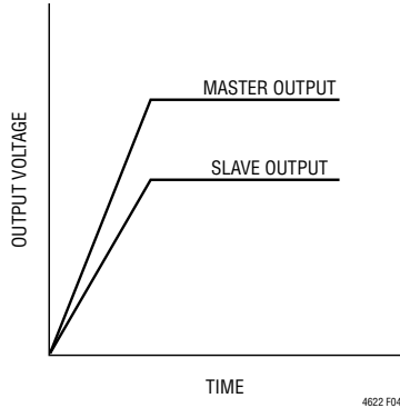
Figure 4. Output Ratiometric Tracking Waveform
