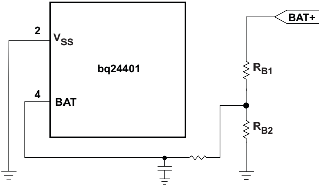
Figure 10. Battery Voltage Divider and Filter
