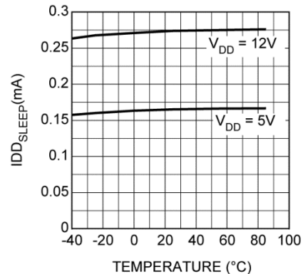
I_{DD\text{SLEEP}} vs. Temperature
