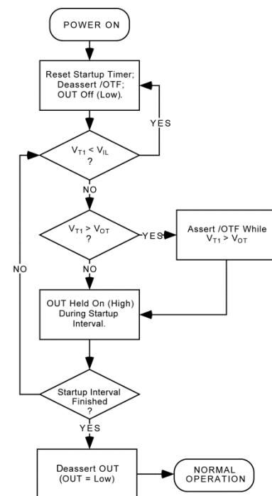
Figure 3. Power-Up Behavior
