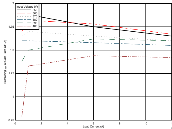
Figure 43. Adaptive Dead-Time
