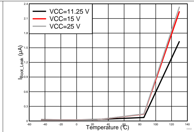
Figure 2. I BOOT_LEAK vs Temperature
