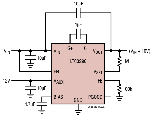
( V_{IN} + 10V ) Tracking Power Supply
