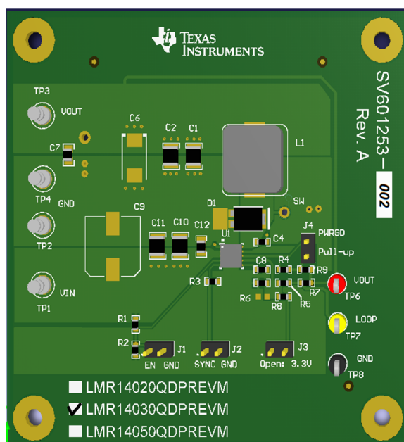
Figure 1. LMR14030QDPREVM Board
