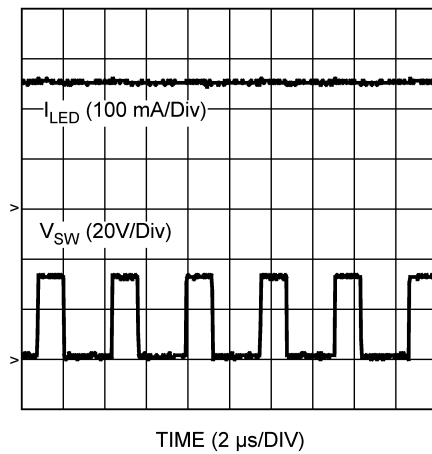
Figure 11. Steady-State Operation
