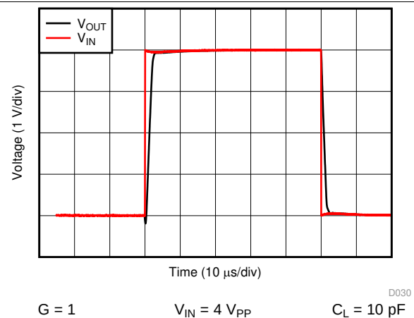
Figure 28. Overload Recovery
