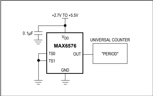
Figure 3. MAX6576 Quick-Look Circuit
