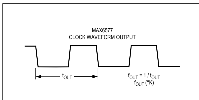
Figure 2. MAX6577 Timing Diagram
