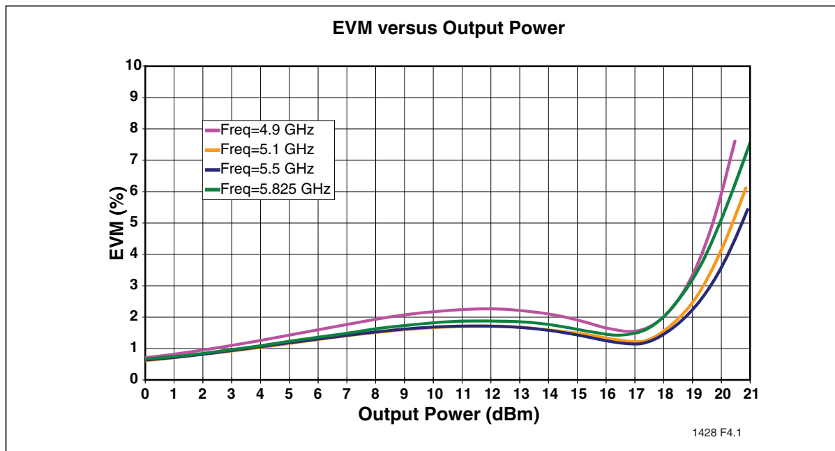
Figure 3: EVM versus Output Power, V_{CC} = 3.3V , V_{REG} = 2.85
