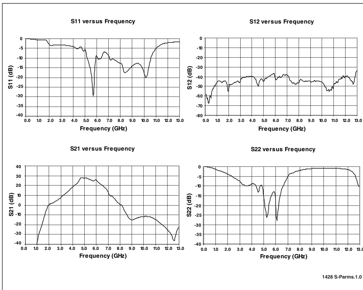
Figure 12: S-Parameters
