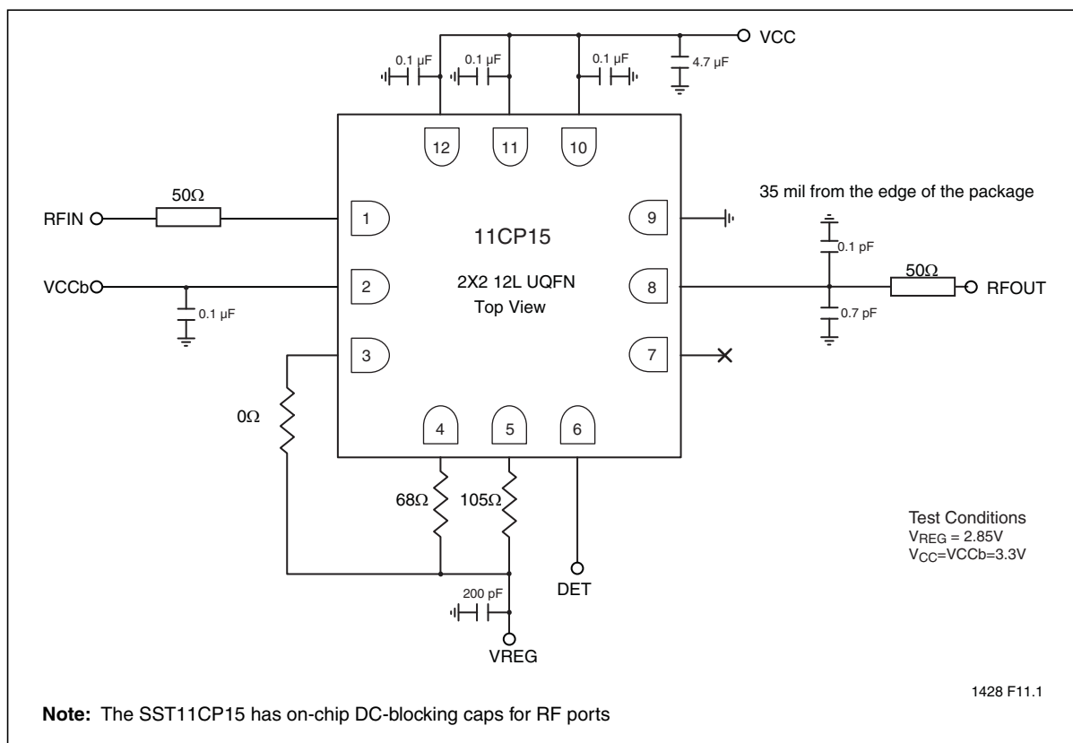
Figure 13: Typical Application for High-Linearity 802.11a/n Application ( V_{CC} = 3.3V , V_{REG} = 2.85V )
