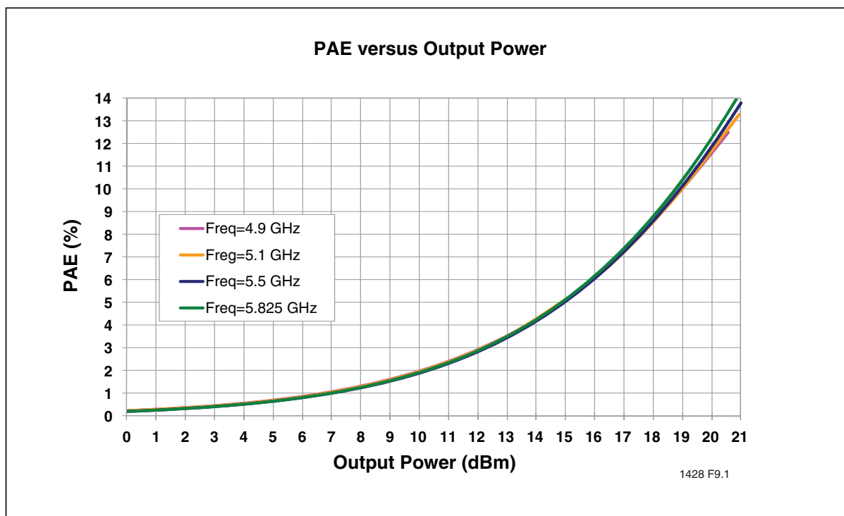
Figure 8: PAE vs Output Power, V_{CC} = 3.3V , V_{REG} = 2.85
