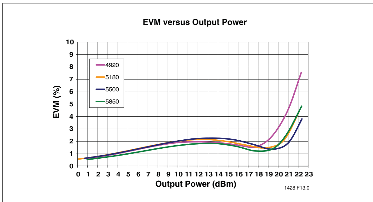
Figure 9: EVM versus Output Power, V_{CC} = 5.0V , V_{REG} = 2.90V
