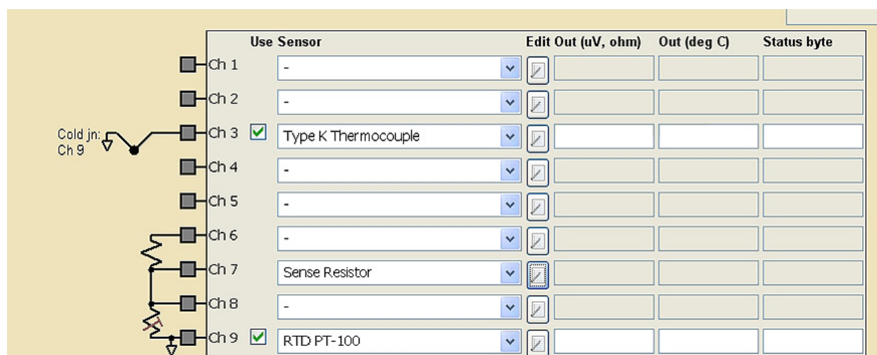
Figure 13. Final Configuration
