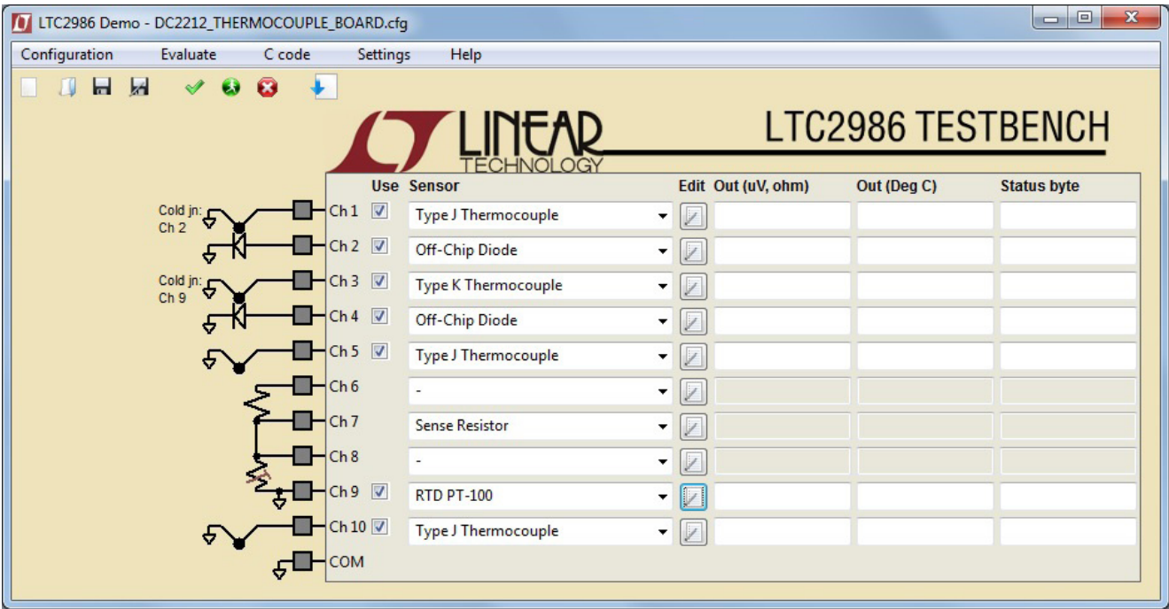
Figure 14. Opening DC2212_THERMOCOUPLE_BOARD.cfg
