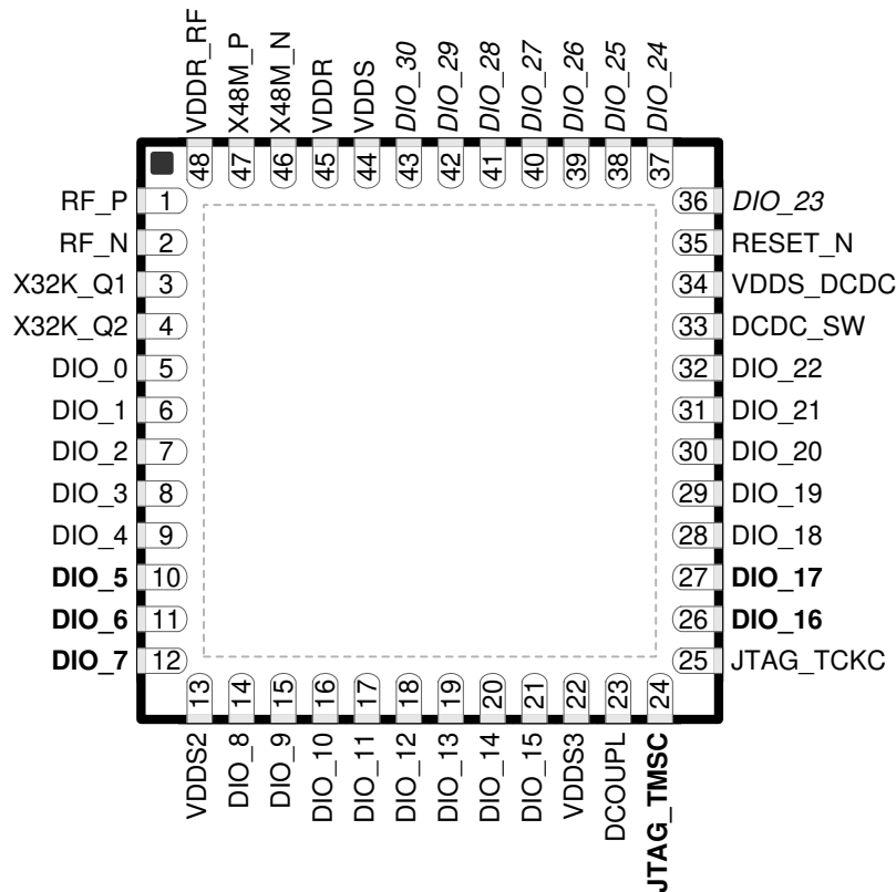
Figure 4-1. RTC (7-mm x 7-mm) Pinout, 0.5-mm Pitch (Top View)
