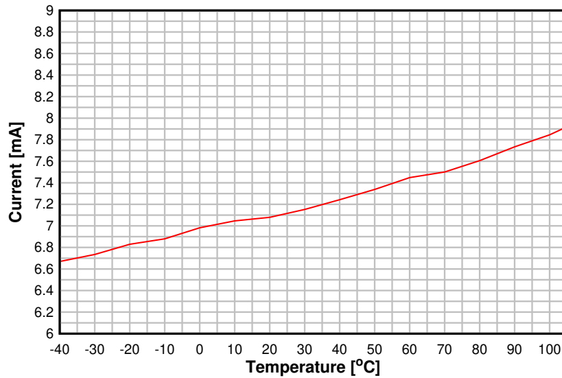
TX Current vs. Temperature BLE 1 Mbps, 2.44 GHz, 0 dBm
