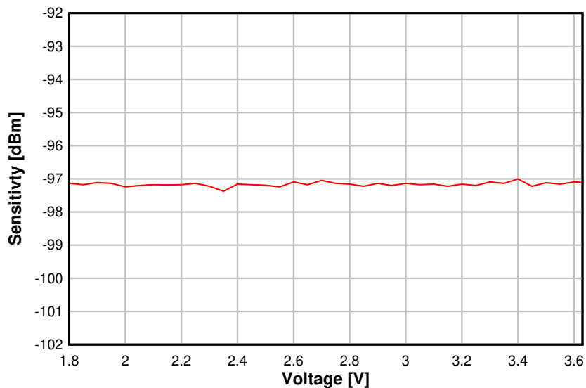
Figure 5-13. Sensitivity vs. Supply Voltage (VDDS) (BLE 1 Mbps, 2.44 GHz)
