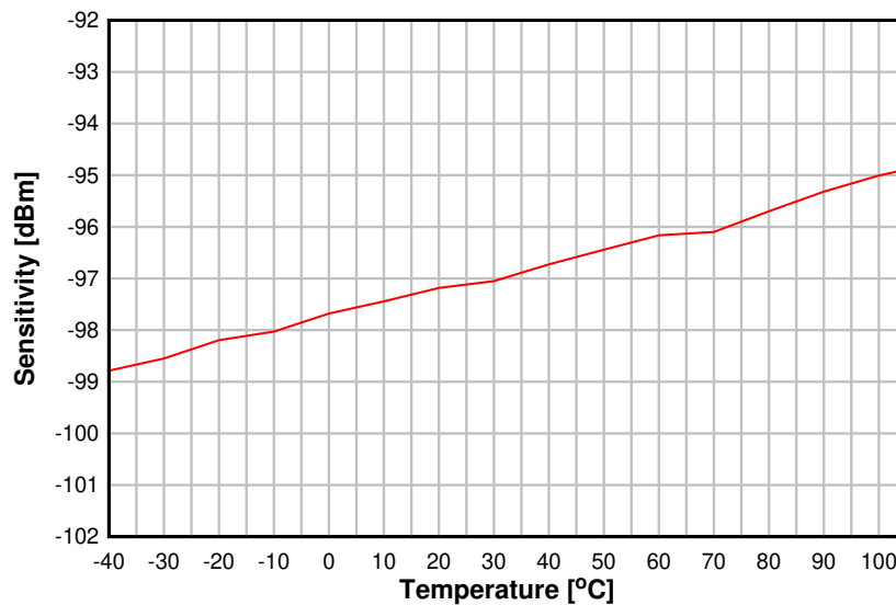
Sensitivity vs. Temperature BLE 1 Mbps, 2.44 GHz
