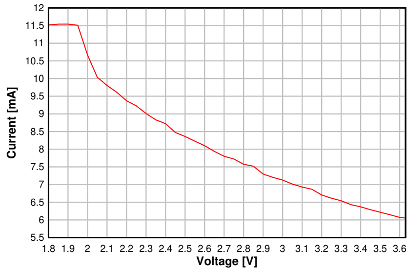
TX Current vs. VDDS BLE 1 Mbps, 2.44 GHz, 0 dBm
