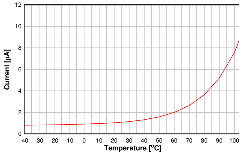
Figure 5-5. Standby Mode (MCU) Current vs. Temperature
