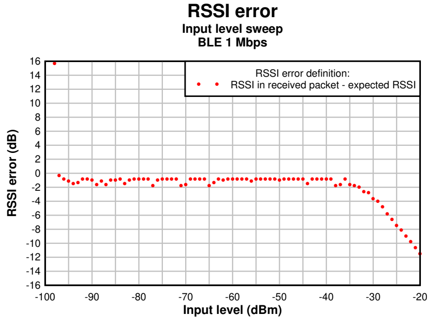
Figure 5-15. RSSI Error vs. Input Level (dBm) (BLE 1 Mbps)
