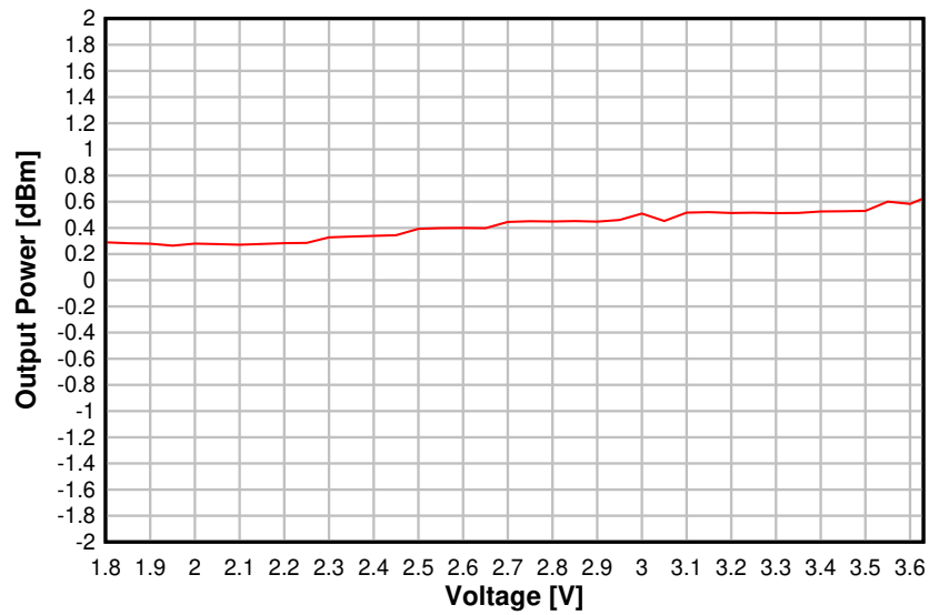
Figure 5-18. Output Power vs. Supply Voltage (VDDS) (BLE 1 Mbps, 2.44 GHz)
