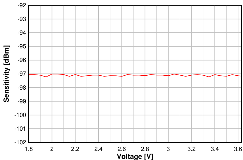
Figure 5-14. Sensitivity vs. Supply Voltage (VDDS) (BLE 1 Mbps, 2.44 GHz, DCDC Off)
