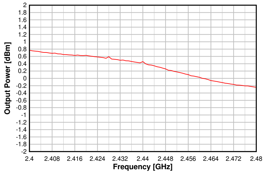
Figure 5-20. Output Power vs. Frequency (BLE 1 Mbps, 2.44 GHz)
