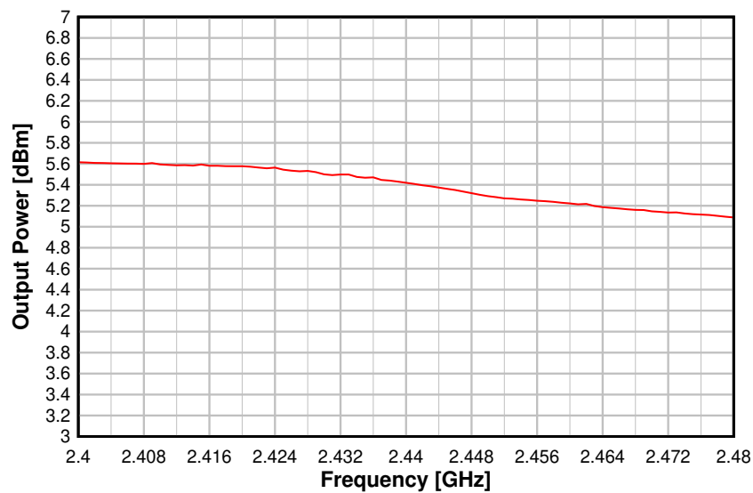
Figure 5-21. Output Power vs. Frequency (BLE 1 Mbps, 2.44 GHz, +5 dBm)
