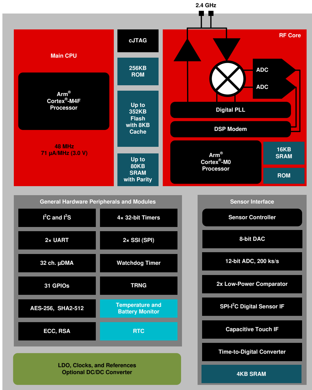
Figure 1-1. CC2642R-Q1 Block Diagram
