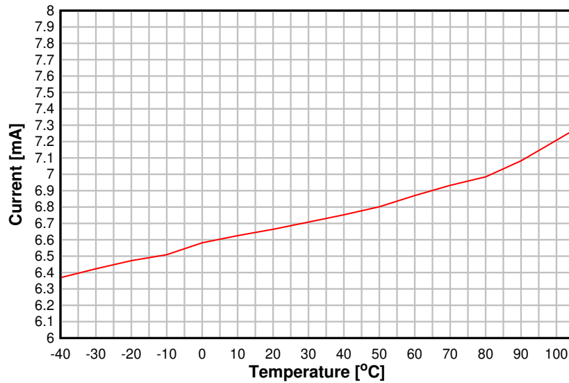
RX Current vs. Temperature BLE 1 Mbps, 2.44 GHz
