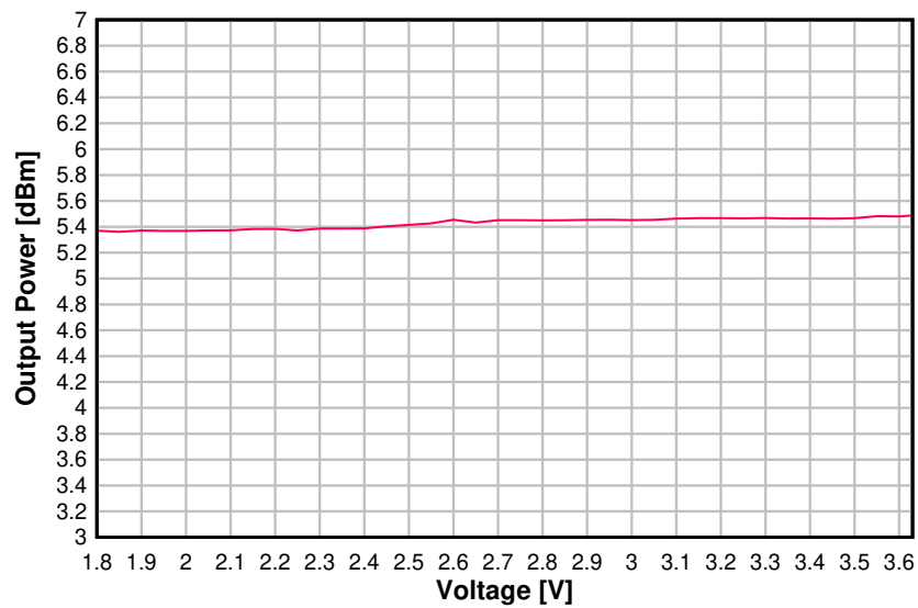
Figure 5-19. Output Power vs. Supply Voltage (VDDS) (BLE 1 Mbps, 2.44 GHz, +5 dBm)
