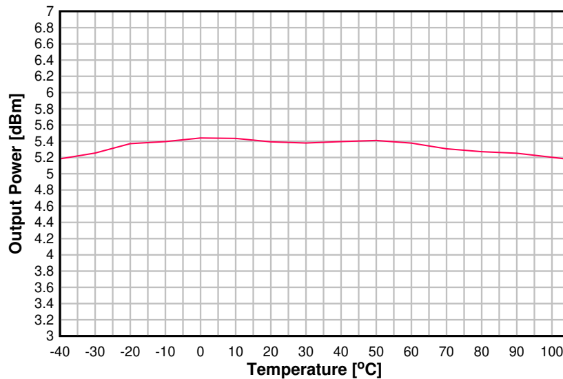
Output Power vs. Temperature BLE 1 Mbps, 2.44 GHz, +5 dBm
