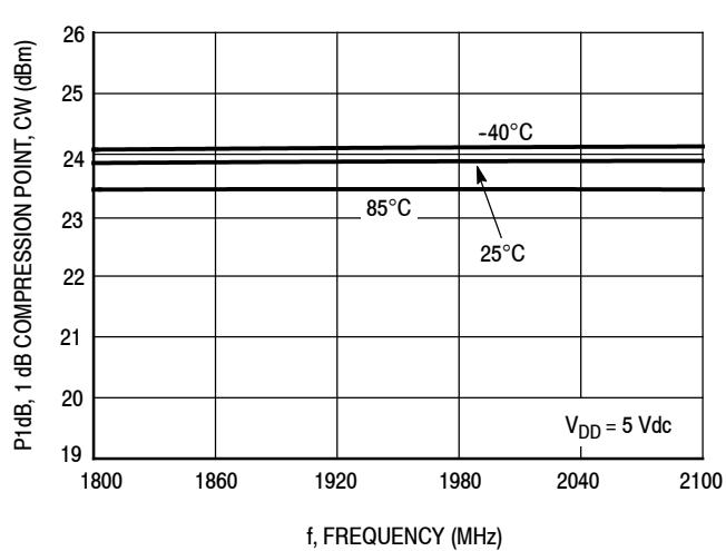
Figure 12. P1dB versus Frequency versus Temperature, CW
