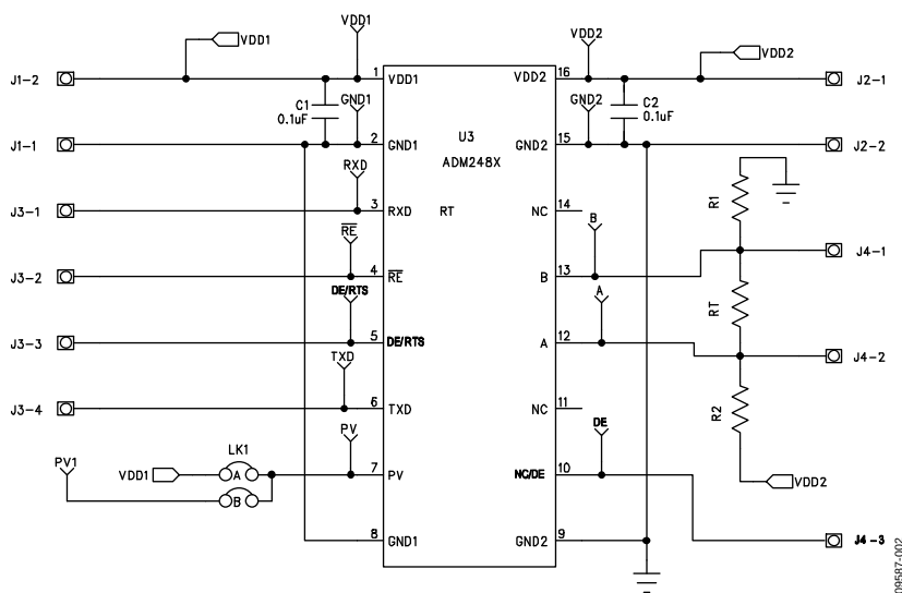
Figure 2. EVAL-ADM2486EBZ Evaluation Board Circuit Diagram
