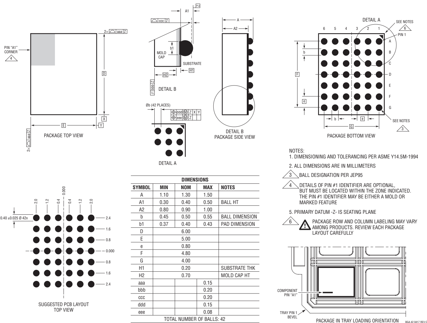
BGA Package 42-Lead (6mm × 5mm × 1.30mm) (Reference ADI DWG # 05-08-1515 Rev C)
