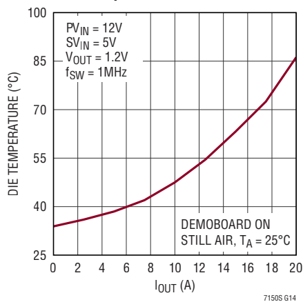
Die Temperature vs Load
