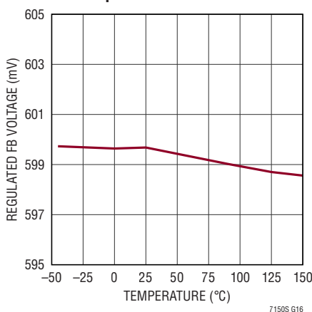
Regulated FB Voltage vs Temperature
