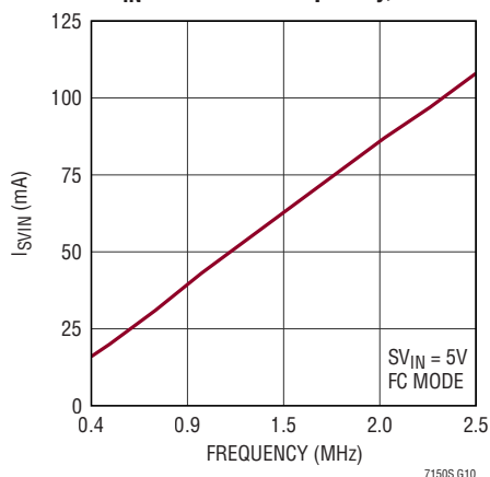
SV IN Current vs Frequency, CCM
