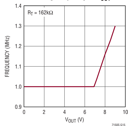
Switching Frequency vs V OUT
