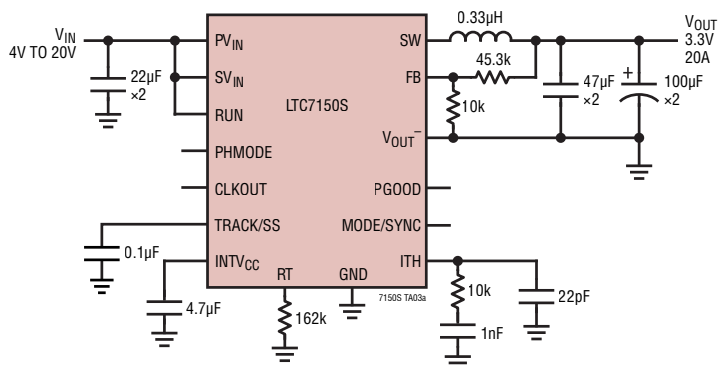
3.3V/20A Step-Down Converter
